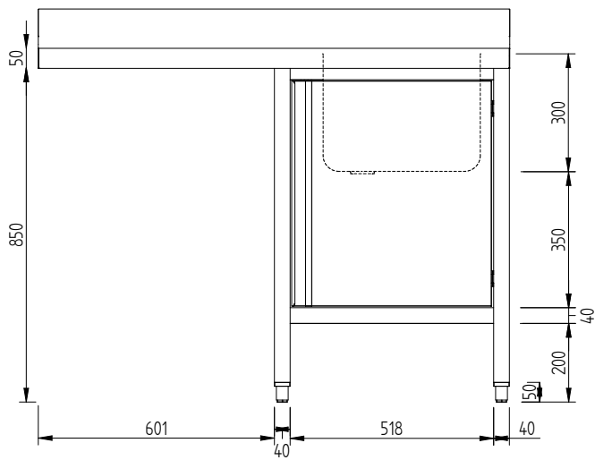
Side
